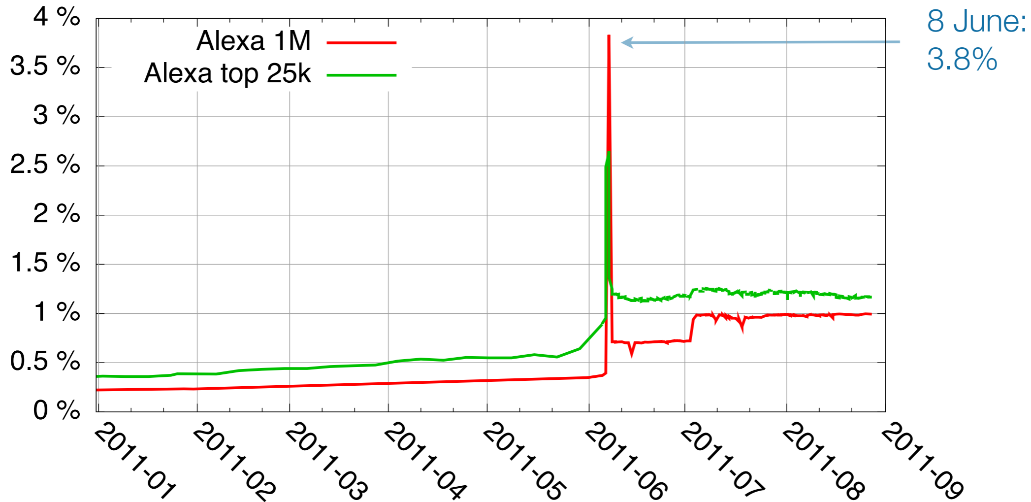
Percentage of web sites in Alexa 1M that can be reached over IPv6
